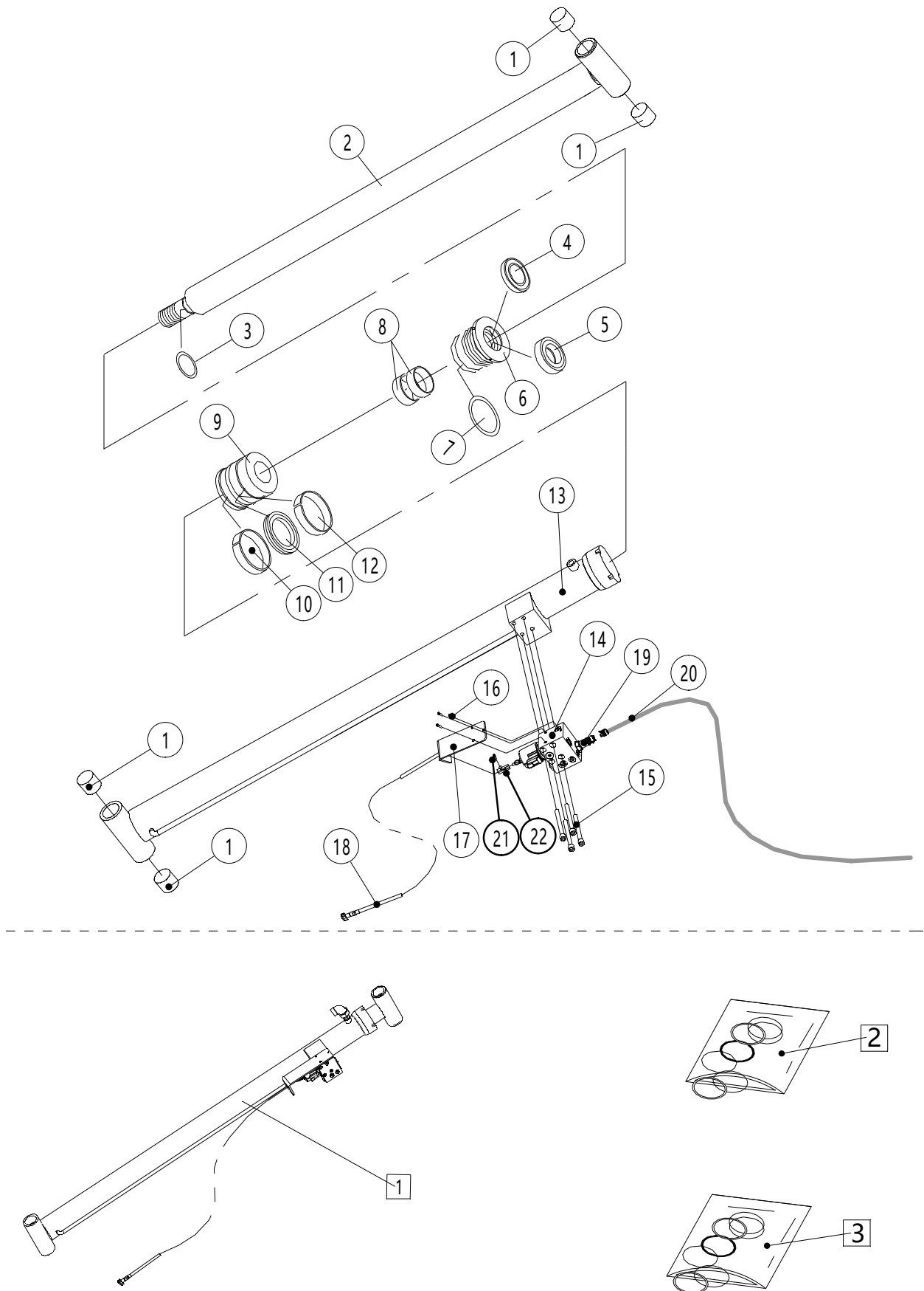
Figure 19 Cylinder
