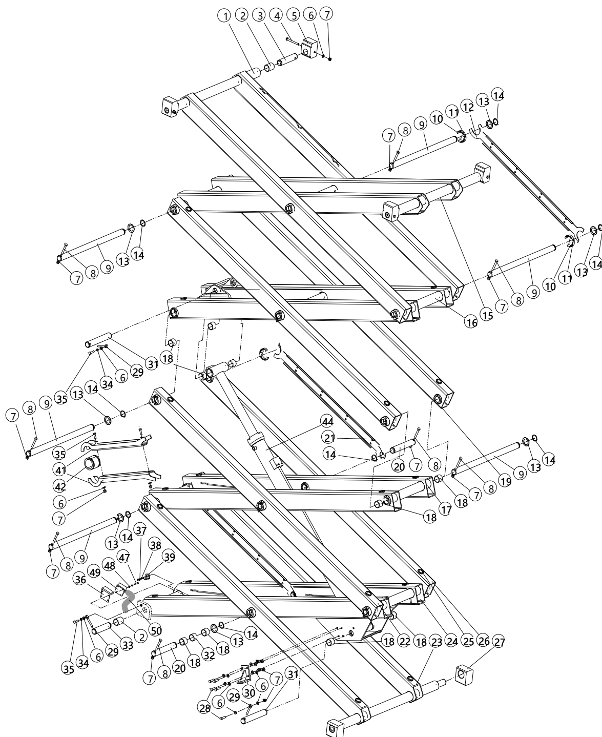
Figure 7 Parts and components of scissors (SC10H/SC10E/SC10H-Li/SC10E-Li)
