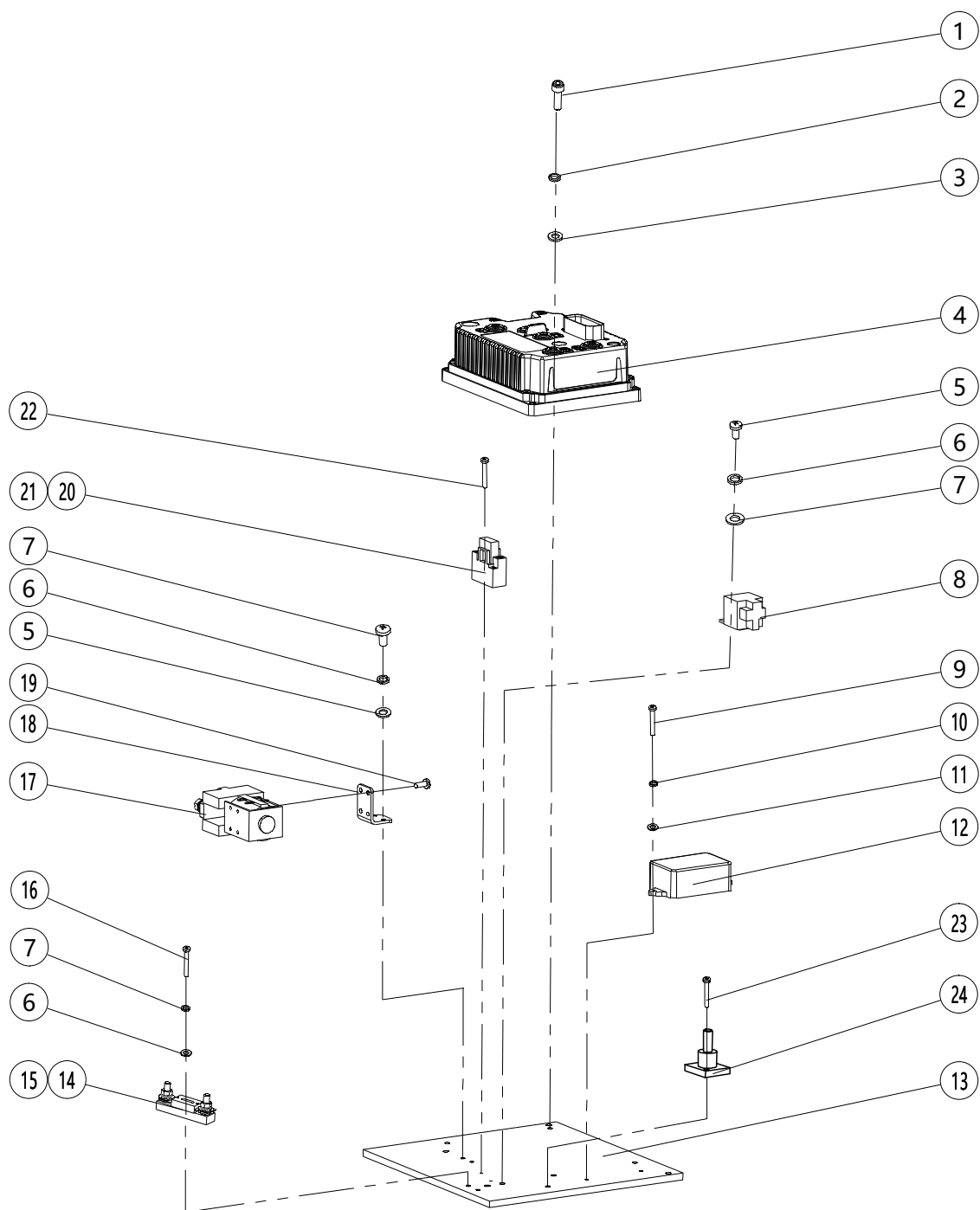
Figure 23 Electrical installation assembly (SC10E/SC12E/SC14E/SC08EN/SC10EN/ SC10E-Li/SC12E-Li/SC14E-Li/SC08EN-Li/SC10EN-Li)
