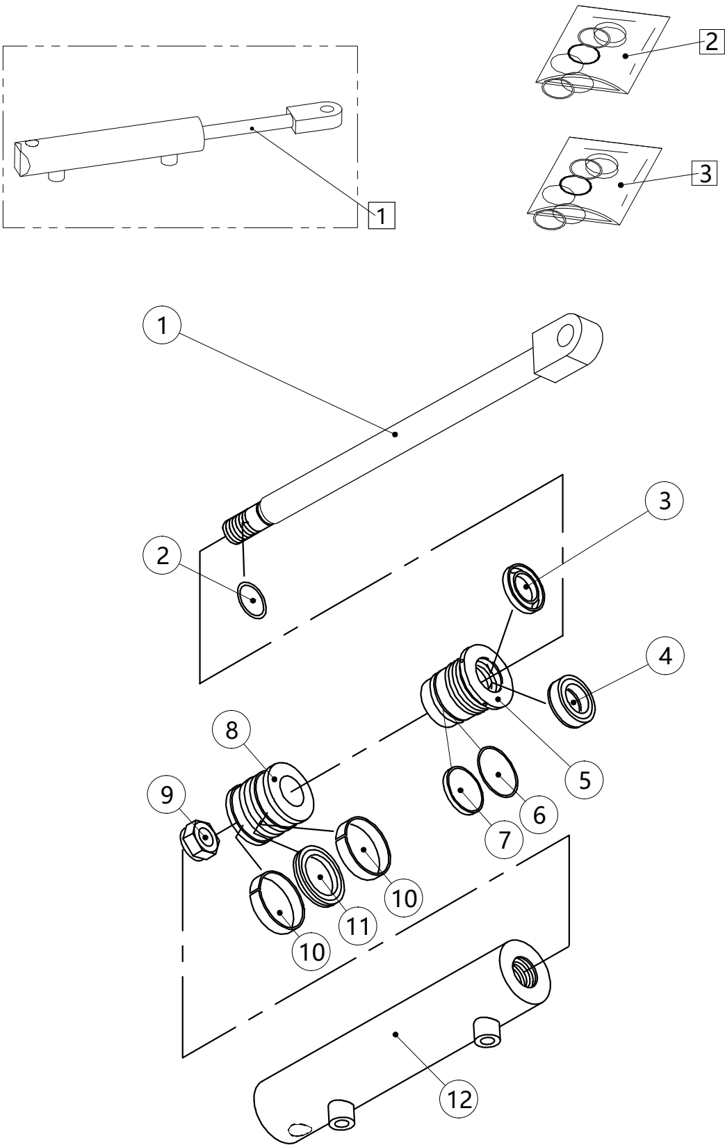
Figure 21 Steering Cylinder
