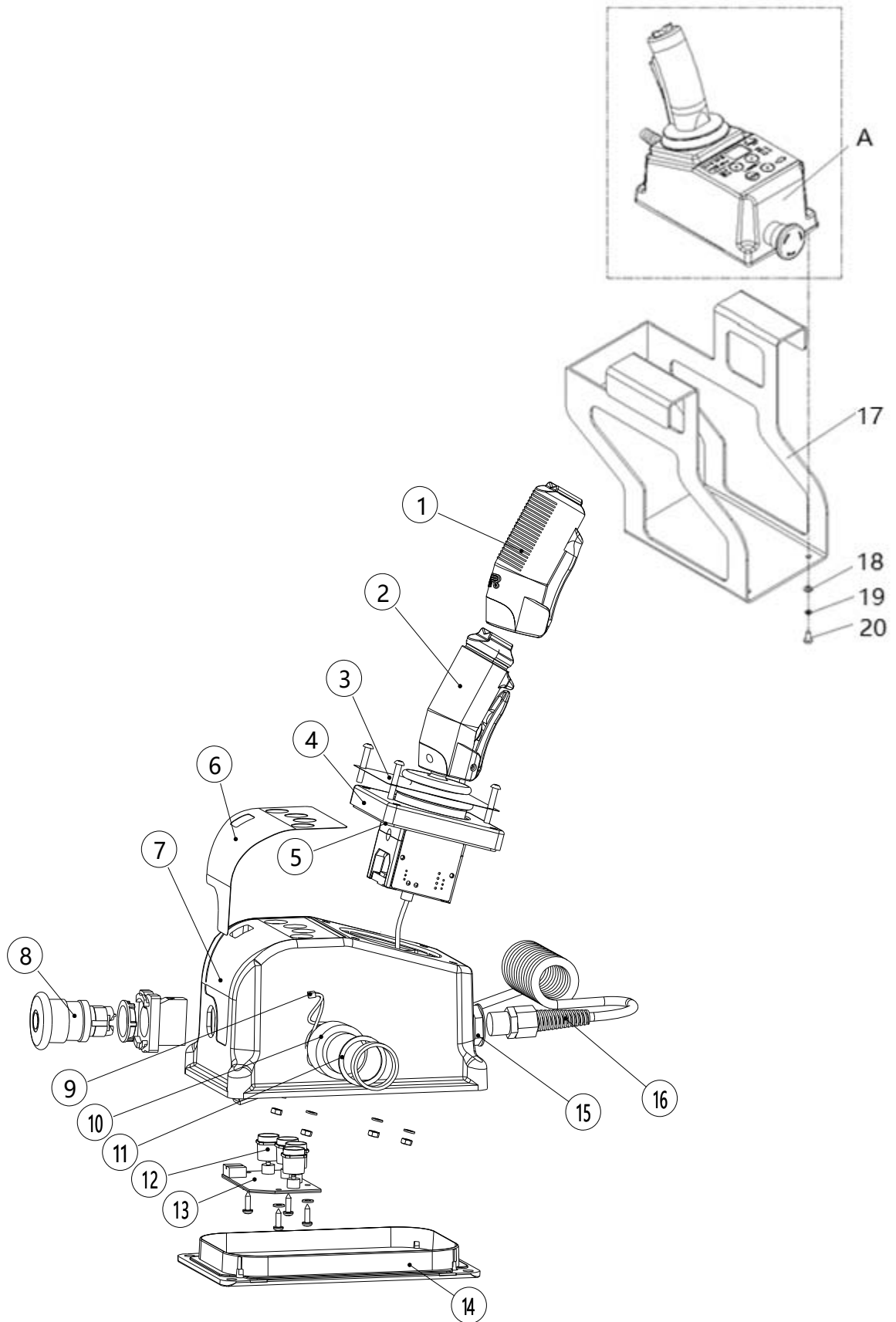
Figure 15 Platform controller components
