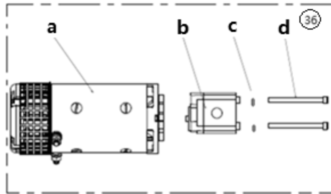
Figure 2.1 Pump station box assembly (SC10H/SC12H/SC14H/SC08HN/SC10HN/ SC10H-Li/SC12H-Li/SC14H-Li/SC08HN-Li/SC10HN-Li)
