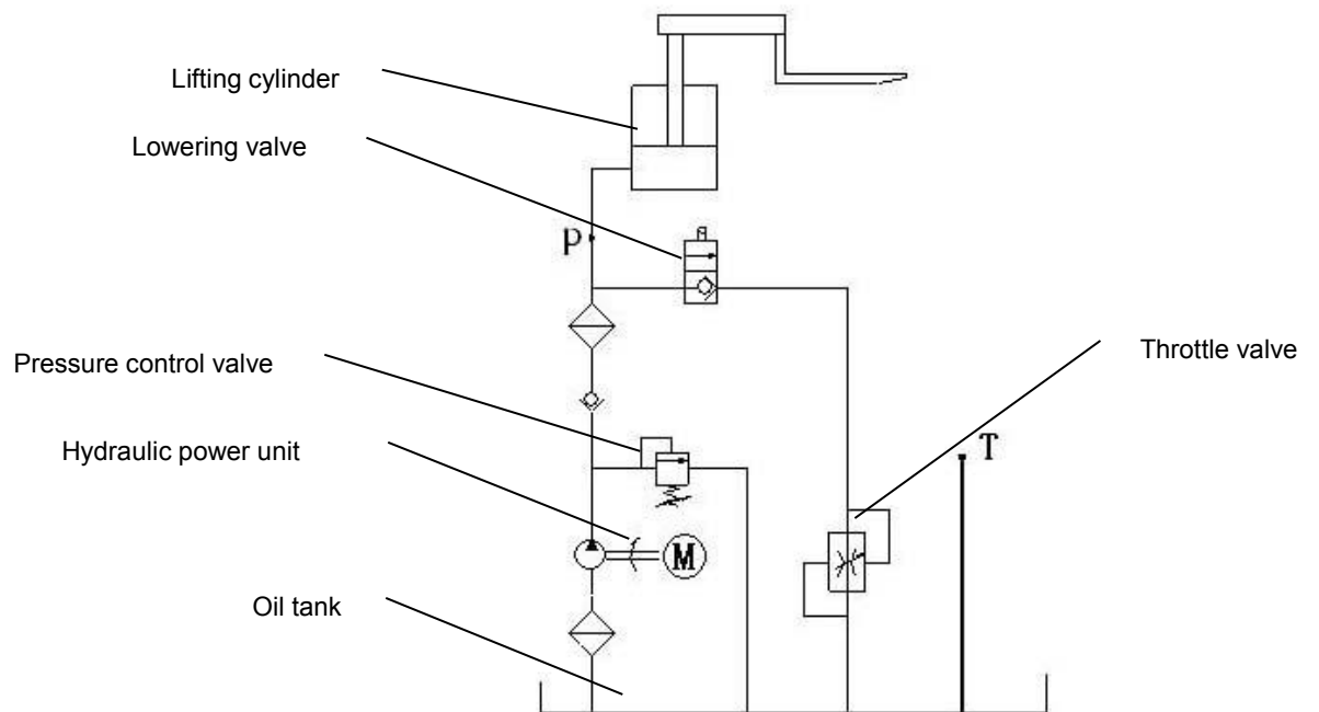
Fig. 20: Hydraulic circuit
